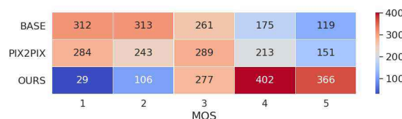
Figure 12. Heatmap of Mean Opinion Score (MOS).
