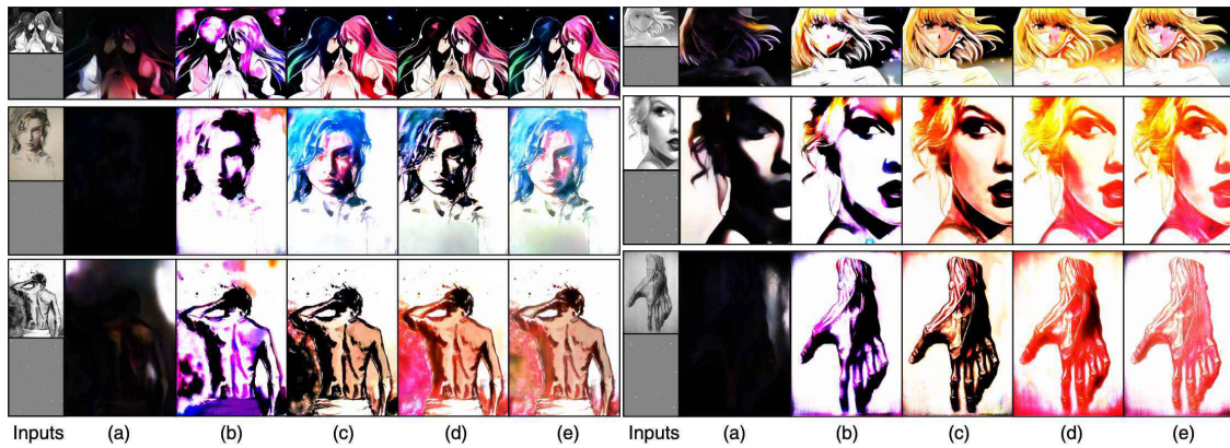
Figure 10. Visual comparison of include grayscale. (a): Base [10], (b): Pix2pix [2], (c): ours (LDM enabled line loss only), (d): ours (histogram equalization only), (e): ours (Both: LDM enabled line loss + histogram equalization).
