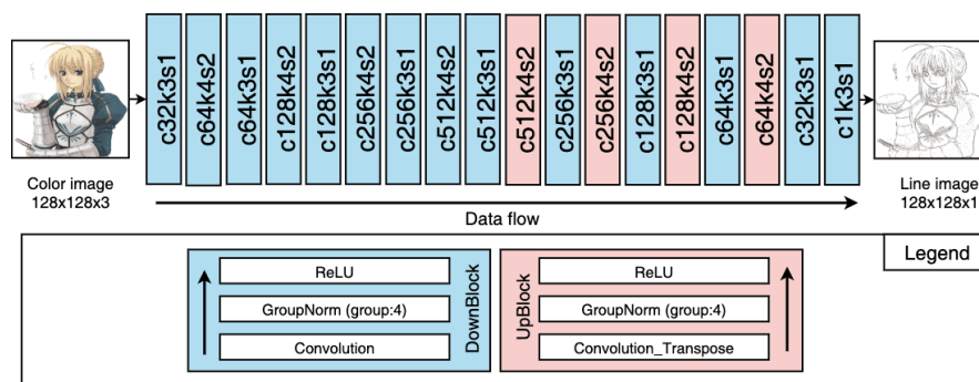
Figure 6. Line Detection Model (c: output filter number, k: kernel Size, s: stride, For example, c32k3s1 means inter convolution layer output filter number is 32, kernel size is 3, and stride is 1).
