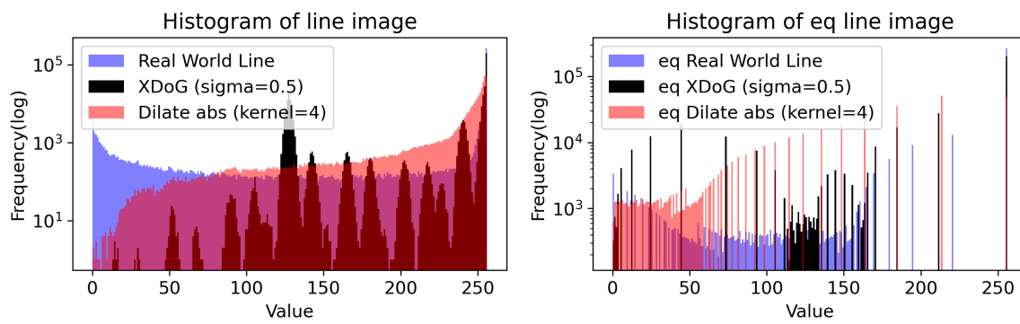
Figure 3. Histogram of line-art (eq: histogram equalization).
