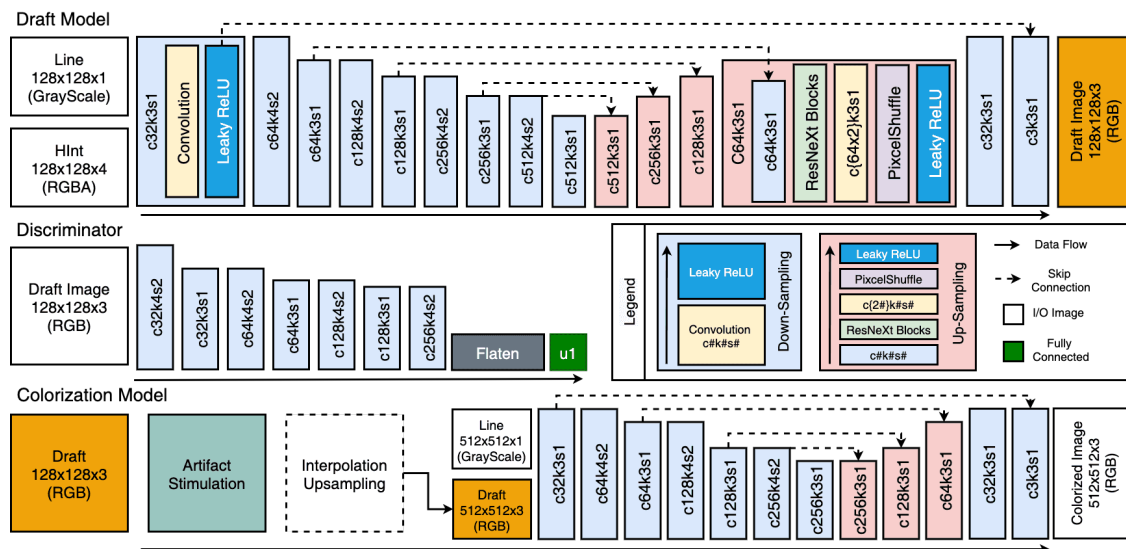
Figure 7. Model architecture (c: output filter number, u: output unit number, k: kernel Size, s: stride).
