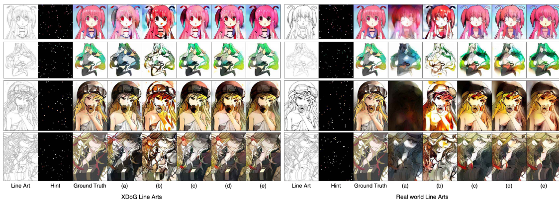
Figure 11. Visual comparison of color restoration (a): Base [10], (b): Pix2pix [2], (c): ours (LDM enabled line loss only), (d): ours (histogram equalization only), (e): ours (Both: LDM enabled line loss + histogram equalization).
