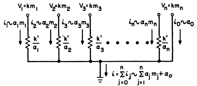
Fig. 2—Implementation of a hyperplane.
