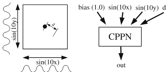
Fig. 11 CPPN periodic inputs. Instead of inputting x and y as usual, \sin(10x) and \sin(10y) are input in the experiments in Sect. 4.4. These inputs create a novel, repeating coordinate frame on which the CPPN can now elaborate. The purpose of this experiment is to show the powerful effect that coordinate transformation can have on phenotypic patterning
