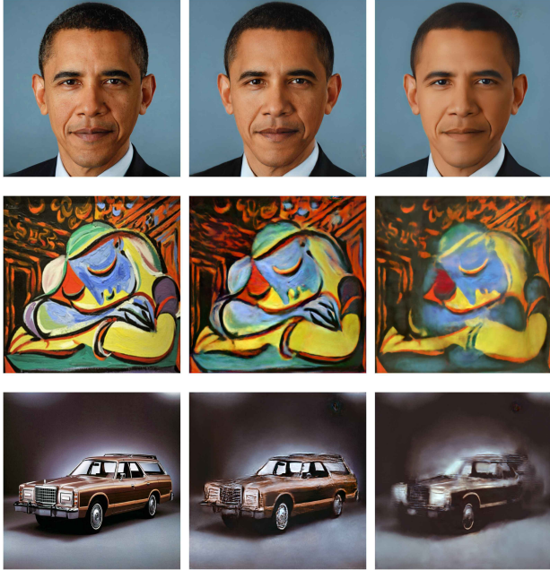
Figure 12: First column: original image ( 1024 \times 1024 ). Second column: embedded image with the perceptual loss applied to resized images of 256 \times 256 resolution. Third column: embedded image with the perceptual loss applied to the images at the original 1024 \times 1024 resolution.
