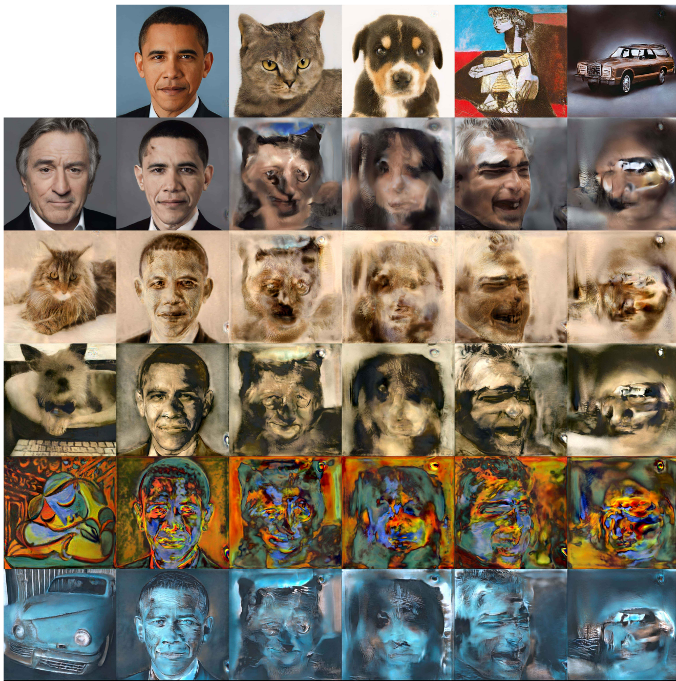
Figure 23: Complete table of the style transfer results. Left-most column: the embedded style image. First row: the embedded content images.
