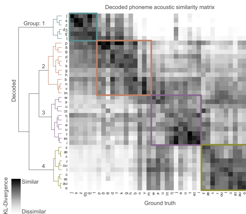
Extended Data Fig. 6 | Decoded phoneme acoustic similarity matrix. Acoustic similarity matrix compares acoustic properties of decoded phonemes and originally spoken phonemes. Similarity is computed by first estimating a Gaussian kernel density for each phoneme (both decoded and original) and then computing the Kullback–Leibler (KL) divergence
