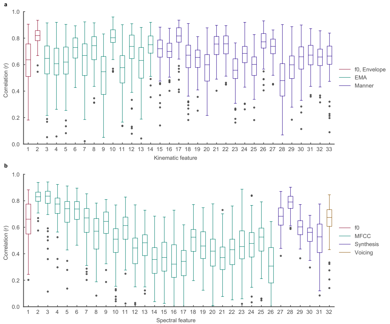
Extended Data Fig. 4 | Decoding performance of kinematic and spectral features. Data from participant 1. a , Correlations of all 33 decoded articulatory kinematic features with ground-truth ( n = 101 sentences). EMA features represent x and y coordinate traces of articulators (lips, jaw and three points of the tongue) along the midsagittal plane of the vocal tract. Manner features represent complementary kinematic features
