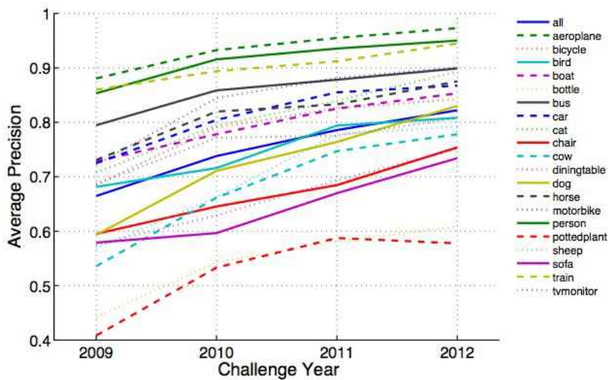
Figure 43: Progress in precision on classification tasks in PASCAL VOC challenges. Reprinted from Williams (2012).
