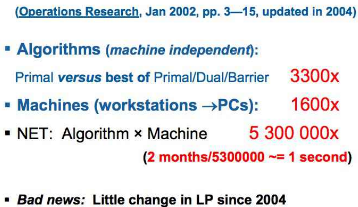
Figure 36: Algorithmic improvement relative to hardware improvement for an unspecified class of linear programming problems. Reprinted from Bixby (2010).
