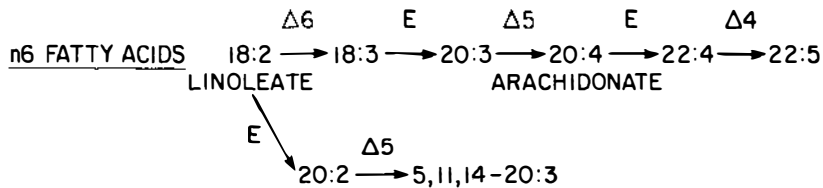
Figure 3 Pathways of linoleate metabolism in mammals. In the liver of the cat there is almost no \Delta 6 -desaturase activity, so arachidonate is a dietary essential. E= elongation, \Delta = desaturation.
