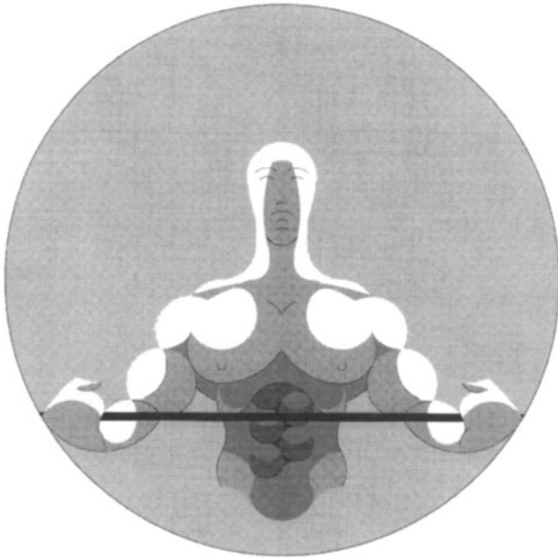
Fig. 4a. Cartoon of a weight lifter's upper body, designed for the logo of a gym. Again, only Rules 1–6 were used to specify the cartoon.
