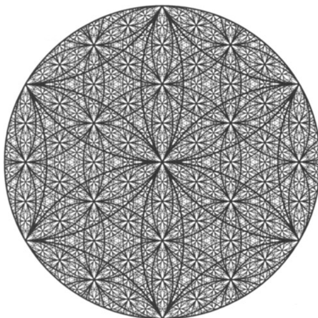
Fig. 1. Fractal result of an iterative application of Rules 1 and 2 (following initialization). This self-similar figure builds the basis of all the figures that follow. On each legal circle there are the centers of six legal circles with equal radius. For clarity, each legal circle is drawn with a width proportional to the logarithm of its radius. Parts of legal circles located outside the initial circle (the “frame”) are not shown. Also, circles with radius less than \frac{1}{16} the radius of the frame are not shown.
