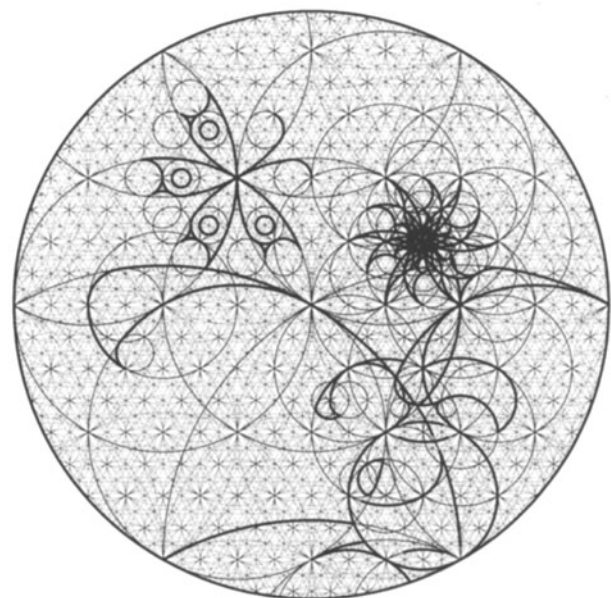
Fig. 2b. Illustration of the low Kolmogorov complexity (or algorithmic simplicity) of Fig. 2a. All circles shown are taken from Fig. 1; very few of them, however, are needed to specify this drawing. Many of the arcs are large and do not require many bits to be specified.
