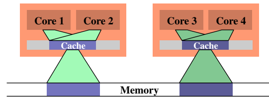
Figure 6.14: Efficient Scheduling
