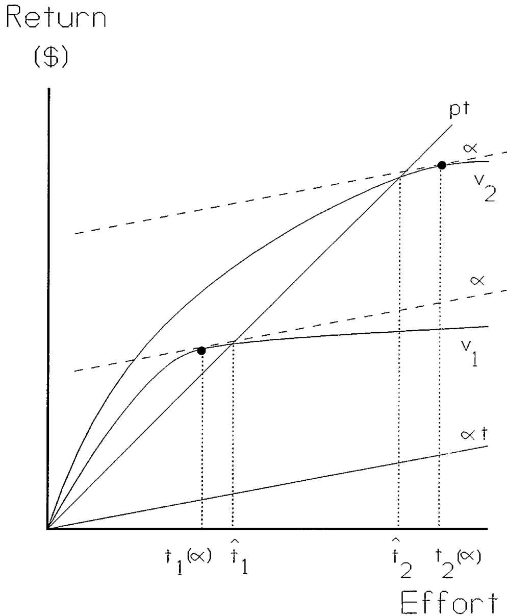
Figure 1. It is optimal to allow task 1 but to exclude task 2, because t_1(\alpha) < \hat{t}_1 but \hat{t}_2 < t_2(\alpha) . Notice that this is true even though the social returns to task 2 are everywhere higher than those to task 1.
