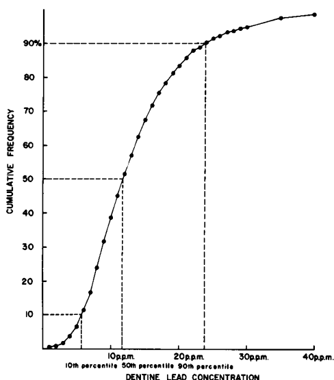
Figure 1. Cumulative Frequency Distribution of Dentine Lead Concentrations (3221 Specimens).
