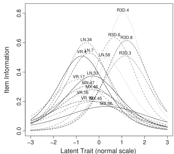
Fig. 4. Item information functions for the 16 item ICAR Sample Test.
