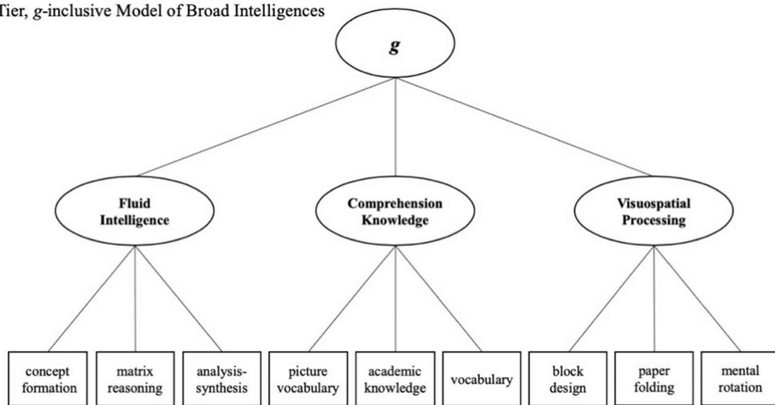
Fig. 1. Comparing two- and three-tier, g-inclusive models of the broad intelligences.
