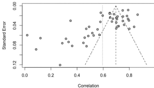
Fig. 4. Funnel plot for meta-analysis exploring the correlation among broad intelligence factors. The dark gray, closed dots represent the observed studies collected in the literature search. The small, dotted vertical line in the plots represents the average, unweighted correlation among broad intelligences at the study level.
