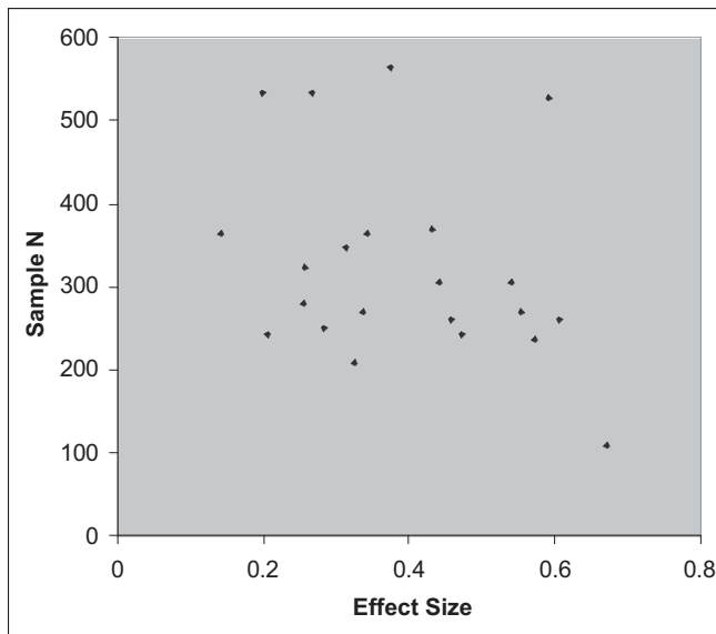
Figure 1 Funnel plot of endpoint effect size as a function of sample size.
