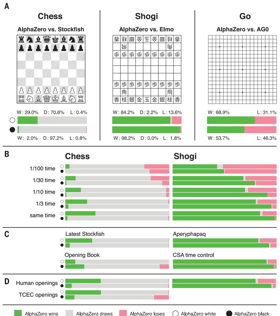
Fig. 2. Comparison with specialized programs. (A) Tournament evaluation of AlphaZero in chess, shogi, and Go in matches against, respectively, Stockfish, Elmo, and the previously published version of AlphaGo Zero (AGO) that was trained for 3 days. In the top bar, AlphaZero plays white; in the bottom bar, AlphaZero plays black. Each bar shows the results from AlphaZero's perspective: win (W; green), draw (D; gray), or loss (L; red). (B) Scalability of AlphaZero with thinking time compared with Stockfish and Elmo. Stockfish and Elmo always receive full time (3 hours per game plus 15 s per move); time for AlphaZero is scaled down as indicated. (C) Extra evaluations of AlphaZero in chess against the most recent version of Stockfish at the time of writing (27) and against Stockfish with a strong opening book (28). Extra evaluations of AlphaZero in shogi were carried out against another strong shogi program, Aperyqhapaq (29), at full time controls and against Elmo under 2017 CSA world championship time controls (10 min per game and 10 s per move). (D) Average result of chess matches starting from different opening positions, either common human positions (see also Fig. 3) or the 2016 TCEC world championship opening positions (see also Fig. S4), and average result of shogi matches starting from common human positions (see also Fig. 3). CSA world championship games start from the initial board position. Match conditions are summarized in tables S8 and S9.
