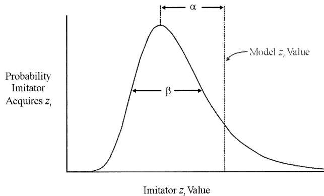
Figure 1. Gumbel distribution for imperfect imitation.
