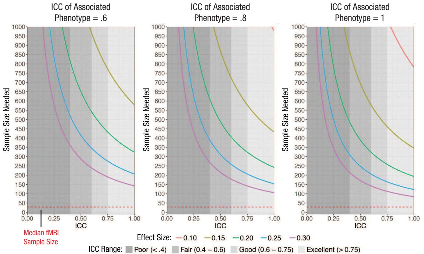
Fig. 1. The influence of task-functional MRI (fMRI) test-retest reliability on the sample size required for 80% power to detect brain-behavior correlations of effect sizes commonly found in psychological research. Power curves are shown for three levels of reliability of the associated behavioral or clinical phenotype. The figure was generated using the pur.r.test function in R (Champely, 2018), with the value for r specified according to the attenuation formula in the Appendix. ICC = intraclass correlation coefficient.
