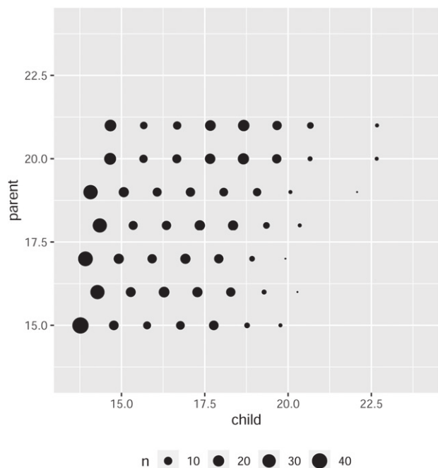
Figure 1. Scatterplot of Galton's peas data. Thickness of a dot represents the number of data points at that location. (Figure courtesy of Susan Holmes.)
