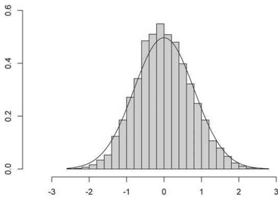
(c) Binomial(3, 0.5), n = 20 .
