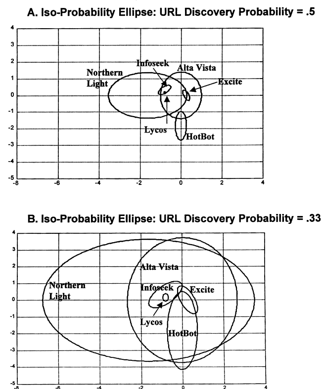
Figure 2 URL Coverage by Six Popular Web Search Engines
