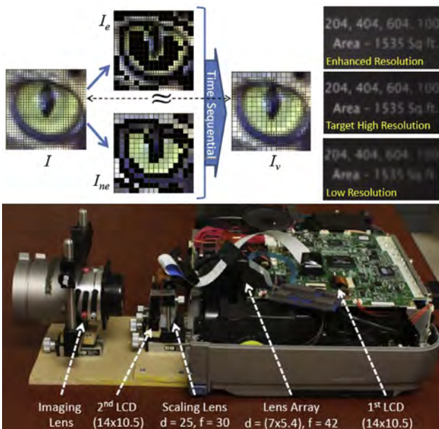
Fig. 15. Spatial resolution enhancement by optical pixel sharing. Top-left: the optical pixel sharing technique decomposes a target high resolution image I into a high resolution edge image I_e and a low resolution non-edge image I_{ne} , which are then displayed in a time sequential manner to obtain the edge-enhanced image I_v . Top-right: comparison of the target image with a low resolution and an enhanced resolution version. Bottom: a side view of the prototype projector, achieving enhanced resolution by cascading two lower-resolution panels [191] (image copyright ACM 2012).
