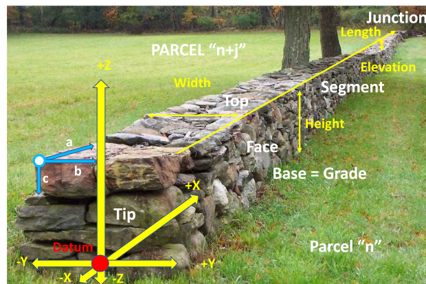
Fig. 4 Coordinate system and terminology for mapping and describing stone walls. Local datum (red dot; X, Y, Z = 0 , 0, 0) is center of base of wall at soil grade at an arbitrary start. Coordinates (yellow arrows) are +X in the forward direction and -X in the reverse direction. Y and Z are orthogonal to X. Elevation anywhere is +/- Z. Wall height at any X is top minus
