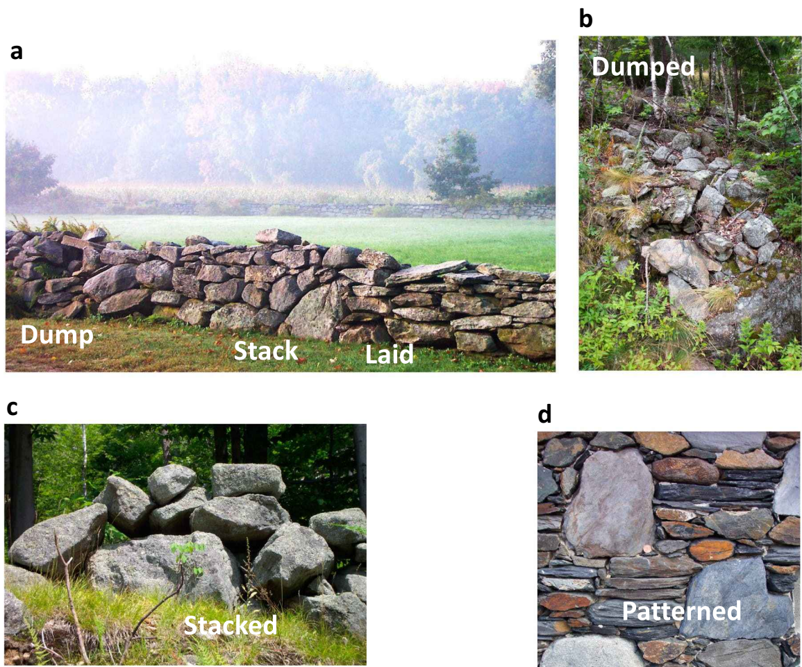
Fig. 9 Examples of degree of order in wall construction. (a) Single wall at Nathan Hale Homestead in Coventry, Connecticut, shows three segments defined by different degrees of order: dumped, stacked, and laid. (b) Wall in Weld, Maine, near the northern end of the common occurrence of New England walls is dumped, a characteristic of pioneering farm-
